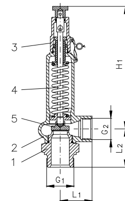
Kopf B / head B
