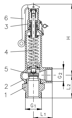
Kopf A / head A
