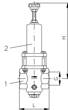
DN 32 – DN 50
