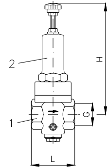
DN 8 – DN 25
